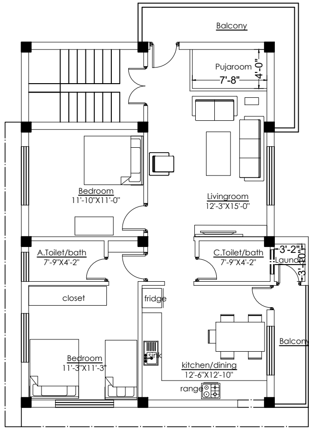
first floor plan plinth area: 975 sqft.
