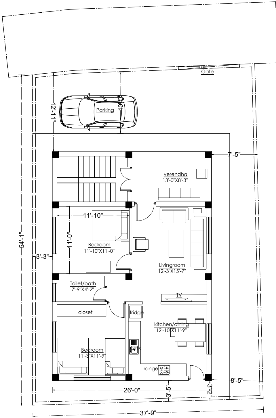
Ground floor plan plinth area: 975 sqft.
